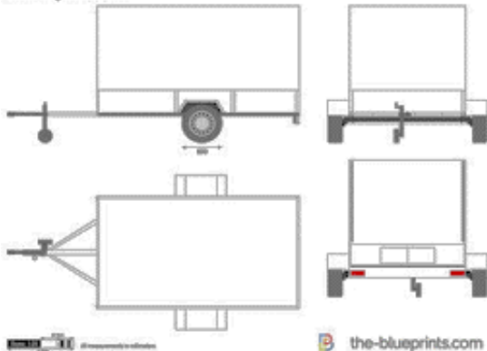
Trailer Single Axle Box v2
